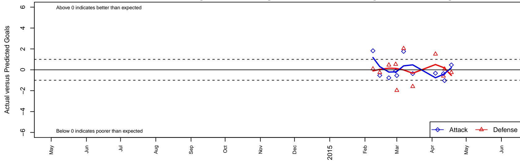
XUnk 4H Bayern Munich G00 Dots are actual minus expected GF (blue circles) and GA (red triangles). Blue line is smoothed change in attack strength. Red is smoothed change in defense strength.
